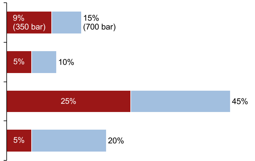
Energy lost in processing and storage In % of energy input
