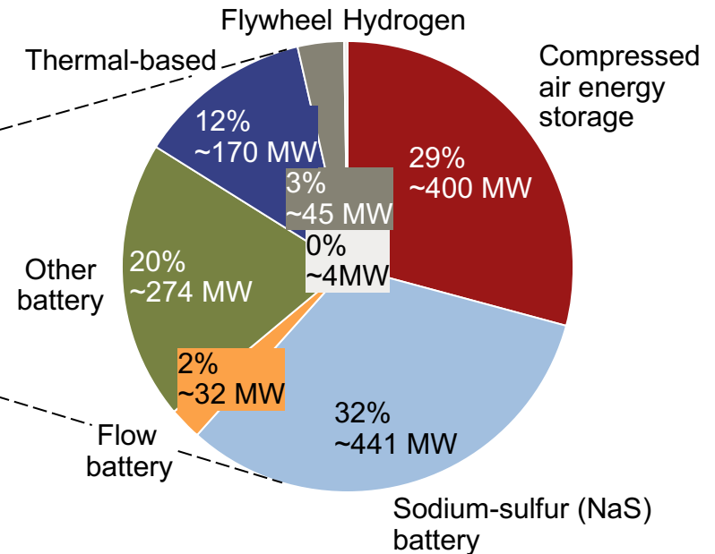
Electricity storage capacity excluding PHS 1 MW, 2012
